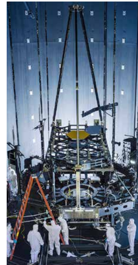
Inside a vacuum chamber at NASA's Johnson Space Center in Houston, the James Webb Space Telescope's Pathfinder backplane test model is being prepared for its cryogenic test. (Photo courtesy of NASA)
